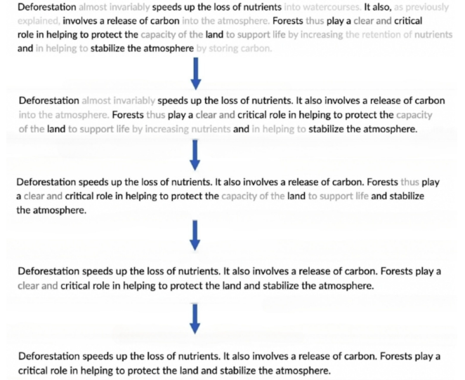
Figure 2: An illustration of how a paragraph shortens with each round of extraction. Each level stays grammatical after shortening. The increasingly faded text at each level before the final most concise extractive summary show what will be removed at each level; the most faded text at the top level was removed first. What is rendered at the top level in this figure is the only rendering of this process that readers see.
